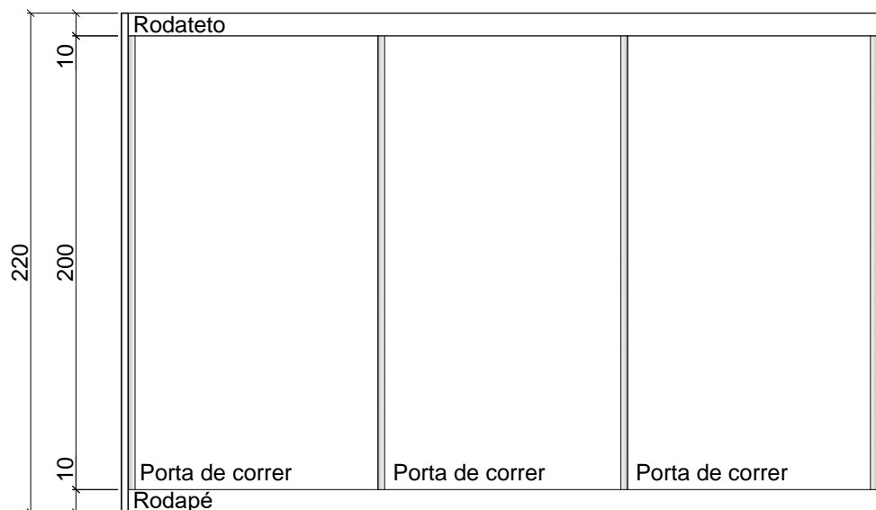
VISTA FRONTAL
